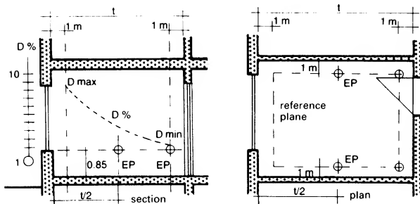
32 Daylight ratio with side lighting, showing the reference plane and the variation in daylight in the internal area
